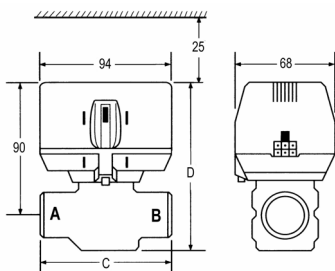
Fig. 1: Dimensions (mm)
